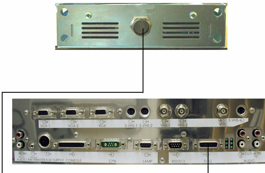
Figure 3-8 ECG Connection Scheme
