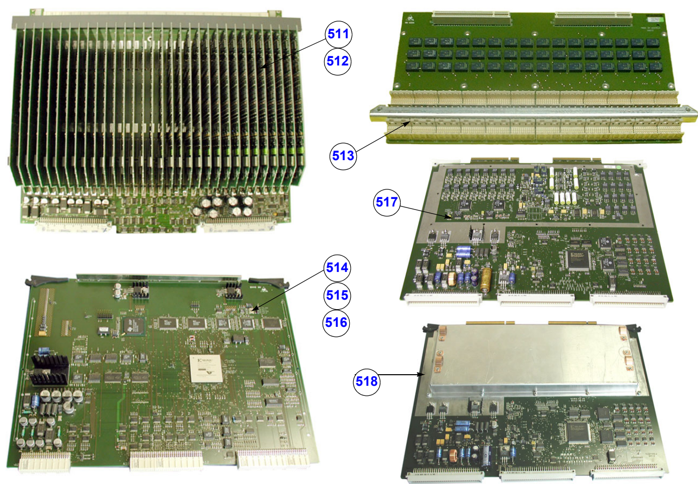
Figure 9-9 FrontEnd (US-Part)
