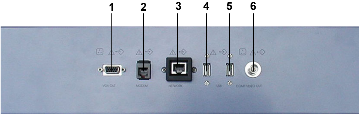
Figure 5-23 External I/O Panel Connectors
