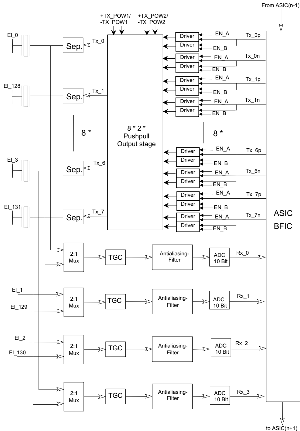
Figure 5-13 Block diagram CPD
