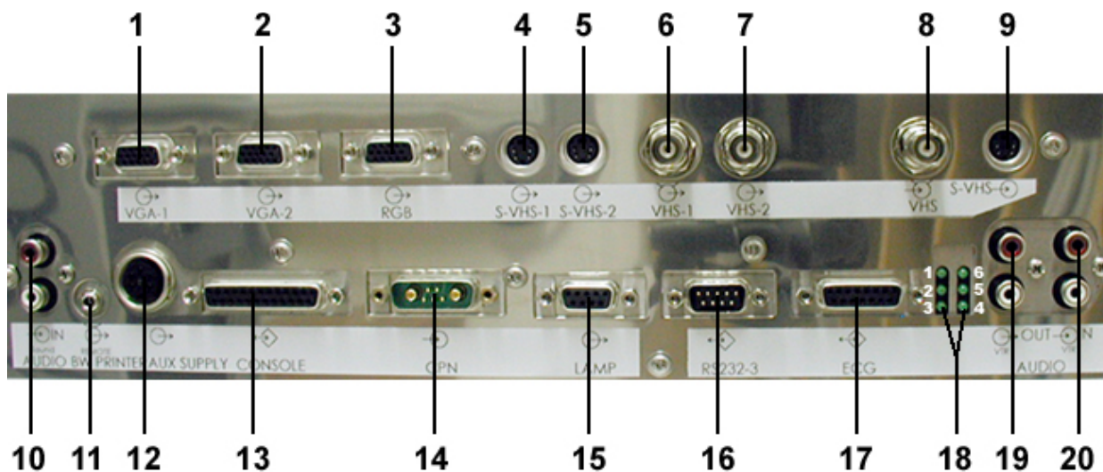
Figure 5-18 Connectors on the Main Module of the GEF
