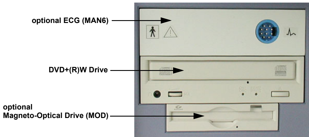
Figure 5-24 GEM incl. optional MOD and ECG
