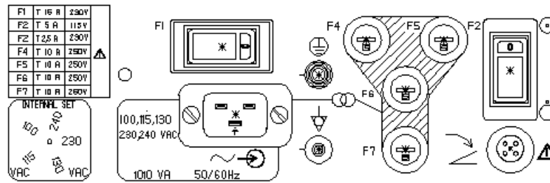
Figure 5-26 Fuses of CPN6
