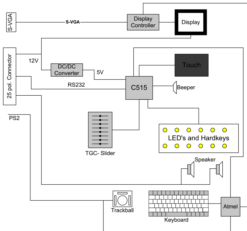
Figure 5-20 Top Console
