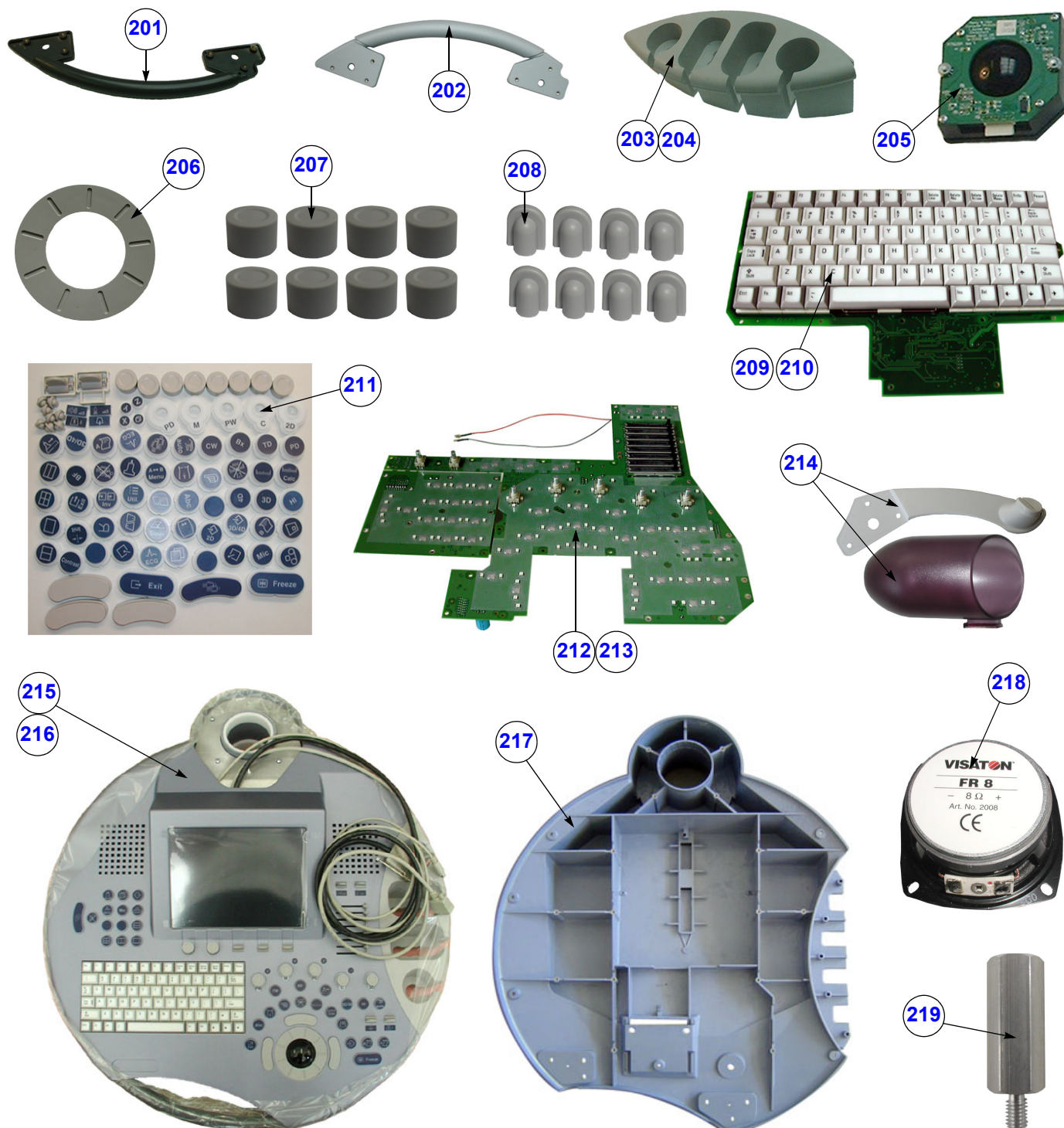
Figure 9-4 User Interface (GEU)
