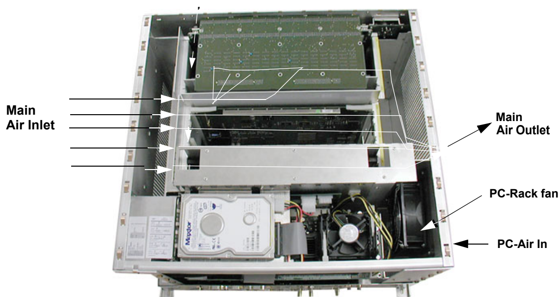
Figure 5-35 Air Flow Control
