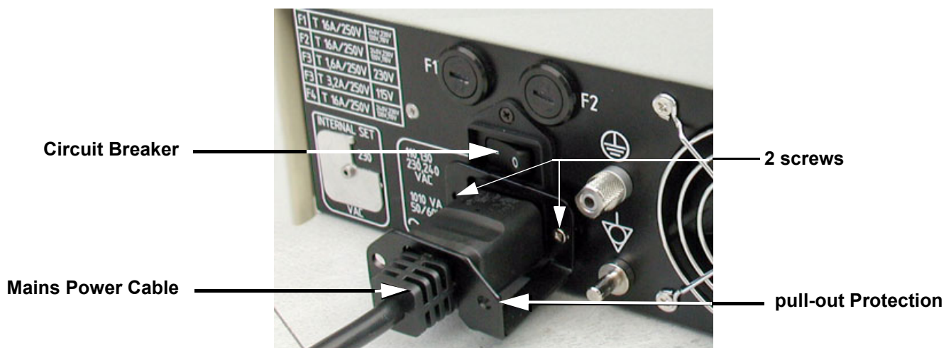
Figure 3-30 Circuit Breaker, Protection and Power Cable on back of Voluson® 730Expert
