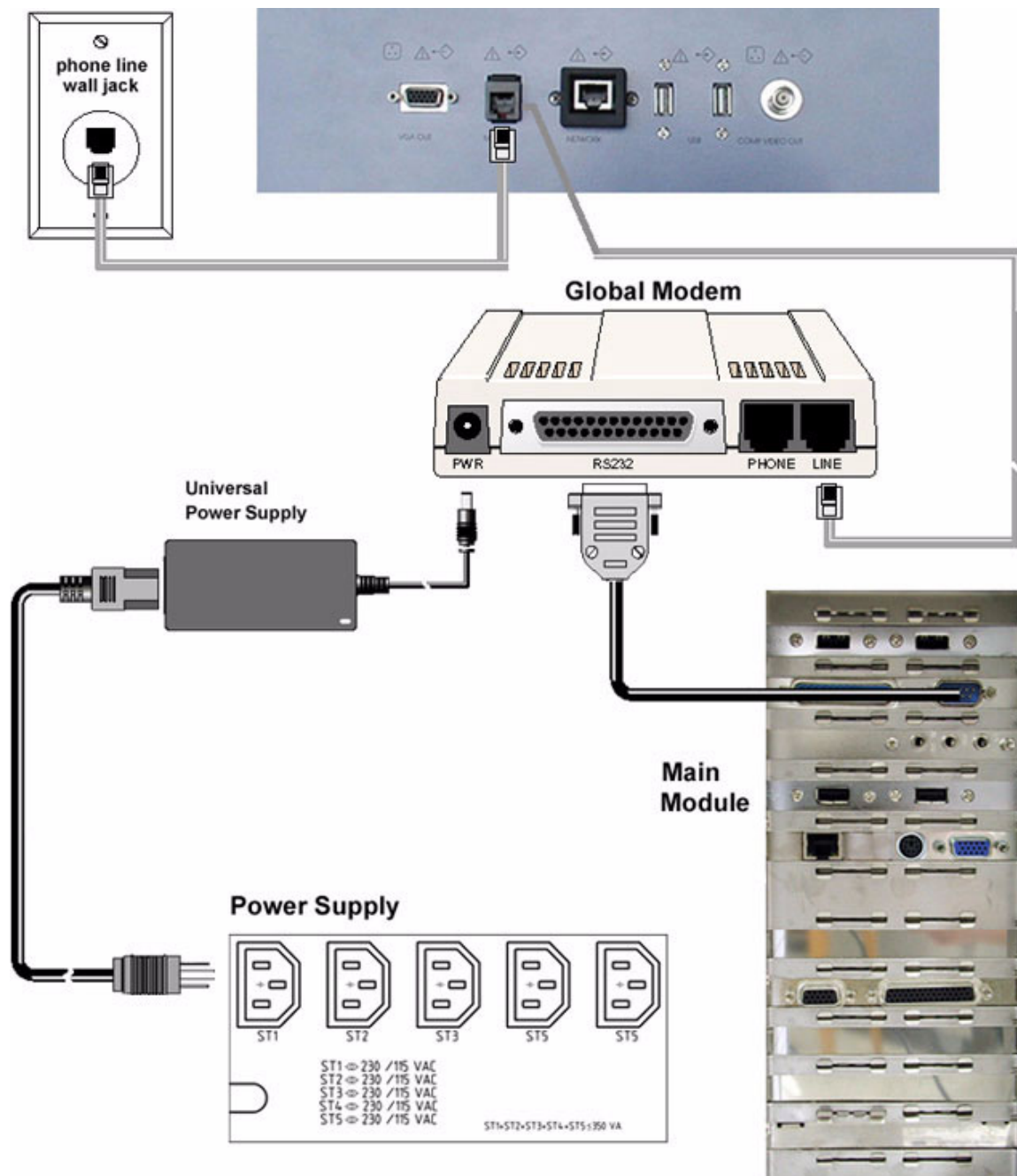
Figure 3-9 Global Modem Connection Scheme
