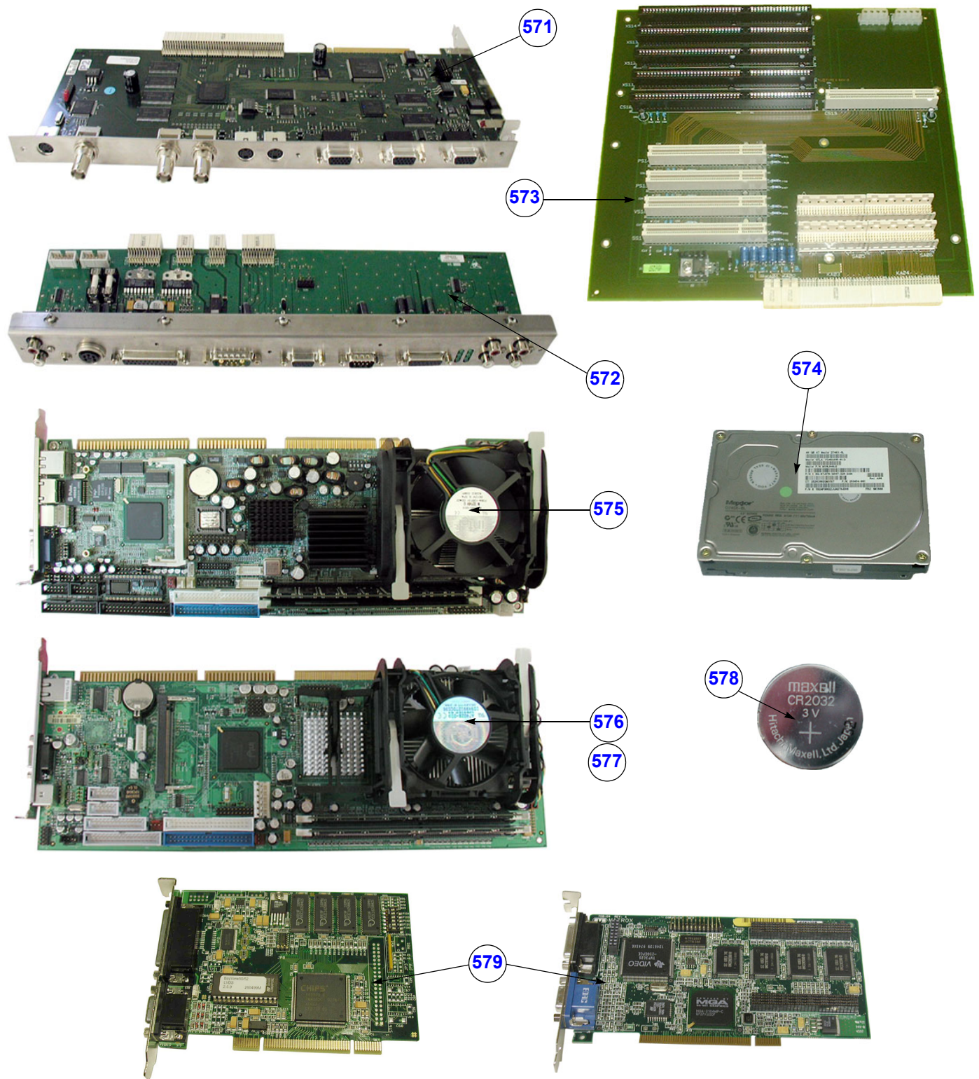
Figure 9-11 Back Processor (PC-Part)
