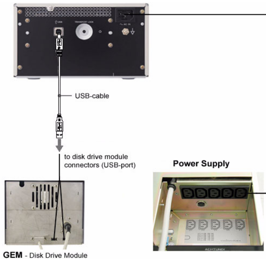
Figure 3-21 Digital Color Printer Connection Scheme
