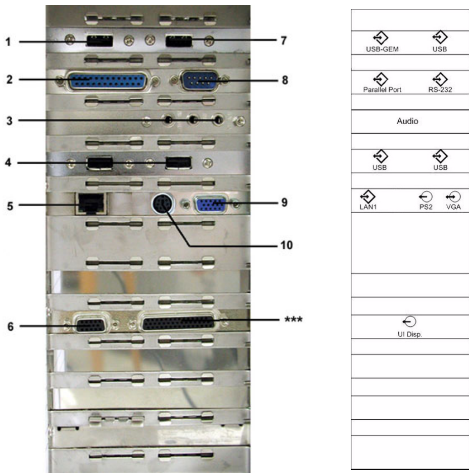
Figure 5-19 Connectors on PC-part of the GEF
