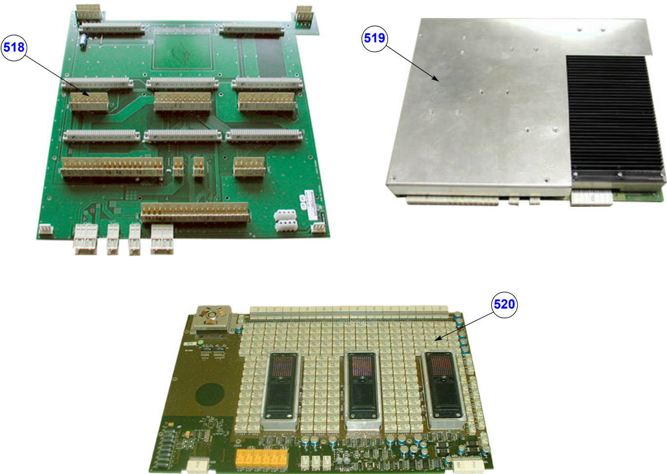
Figure 9-10 FrontEnd (US-Part) cont'd
