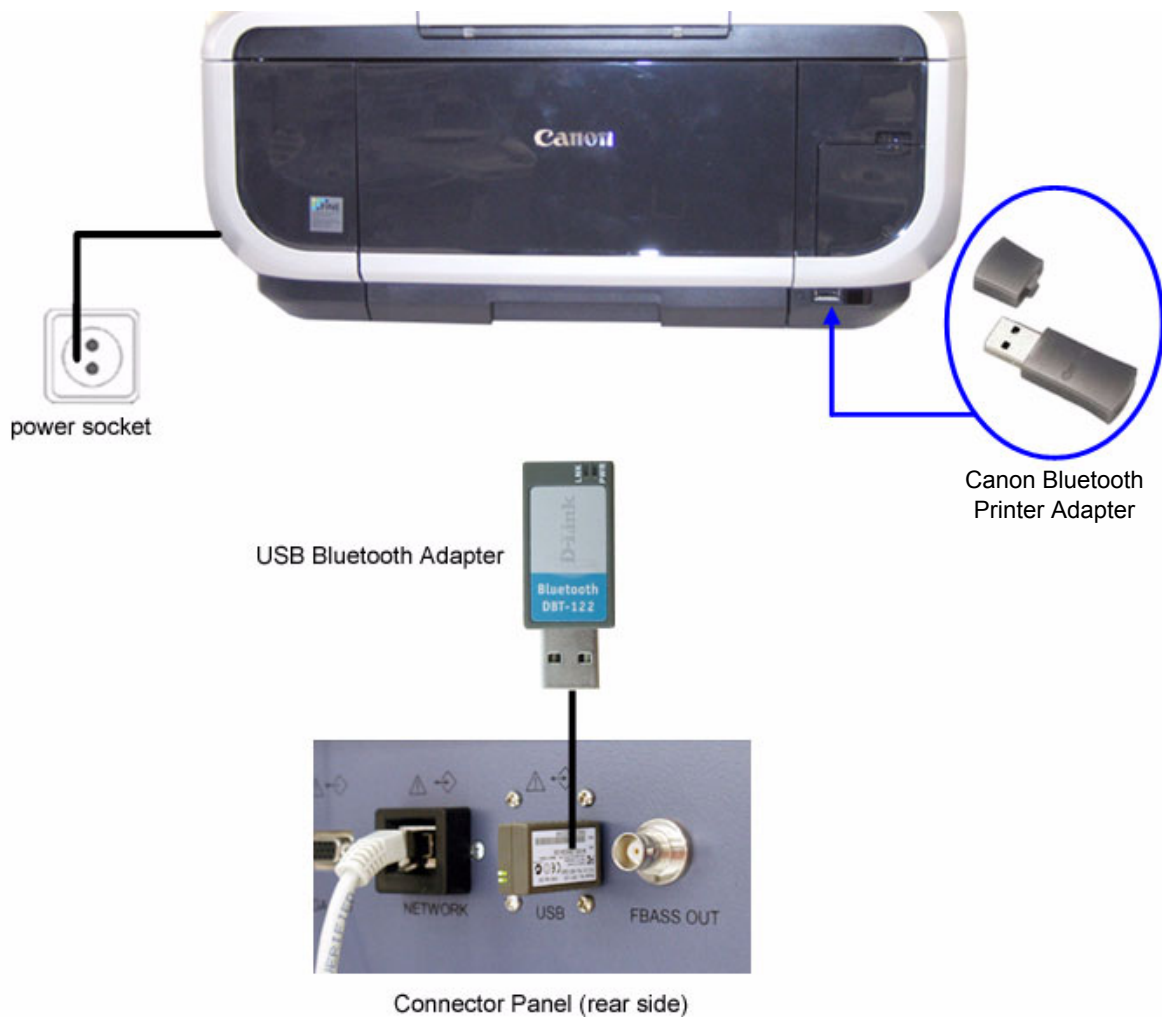
Figure 3-23 Canon Bluetooth Printer - Connection Scheme
