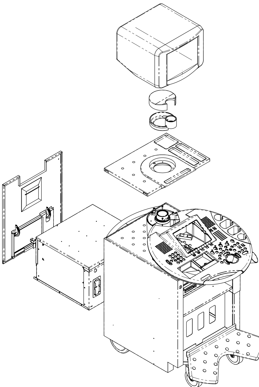
Figure 5-33 Assembly Drawing Voluson® 730Expert
