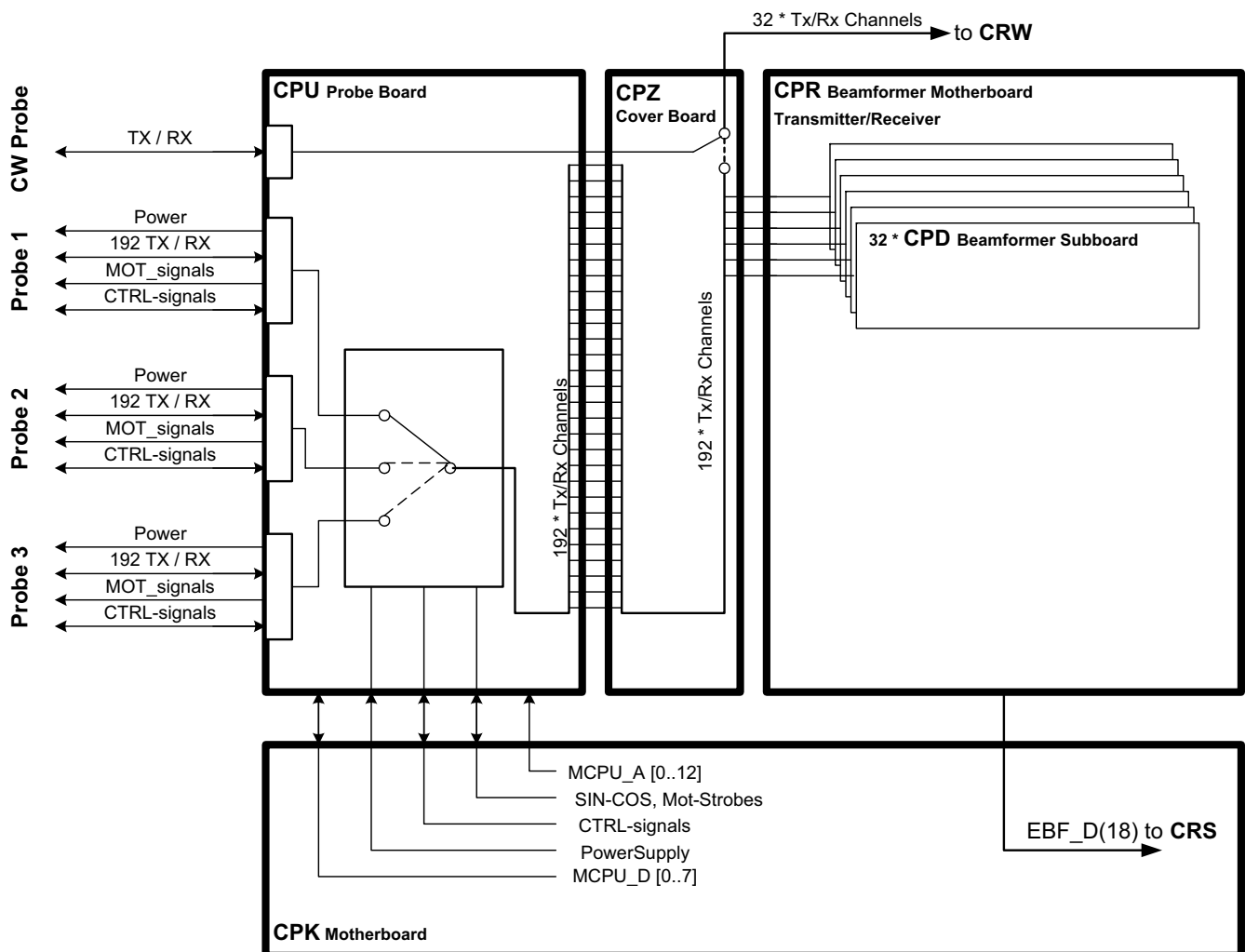
Figure 5-12 CPU + Beamformer (CPR)
