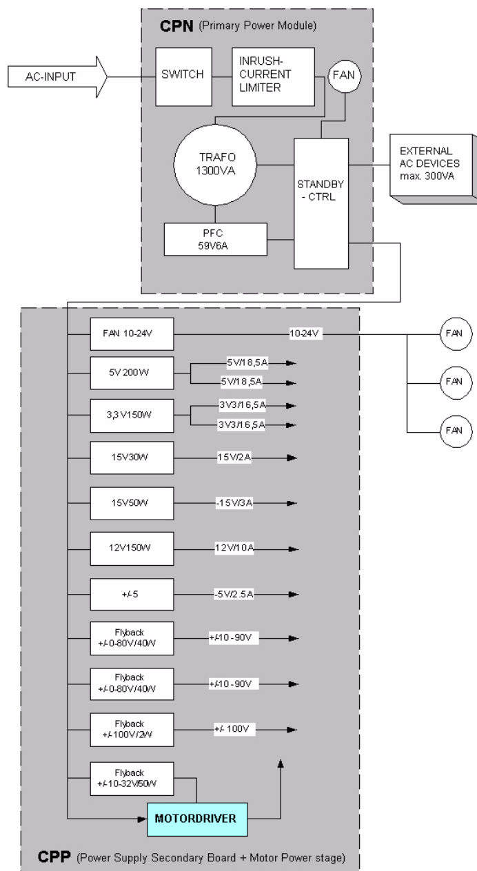
Figure 5-14 Block diagram CPP
