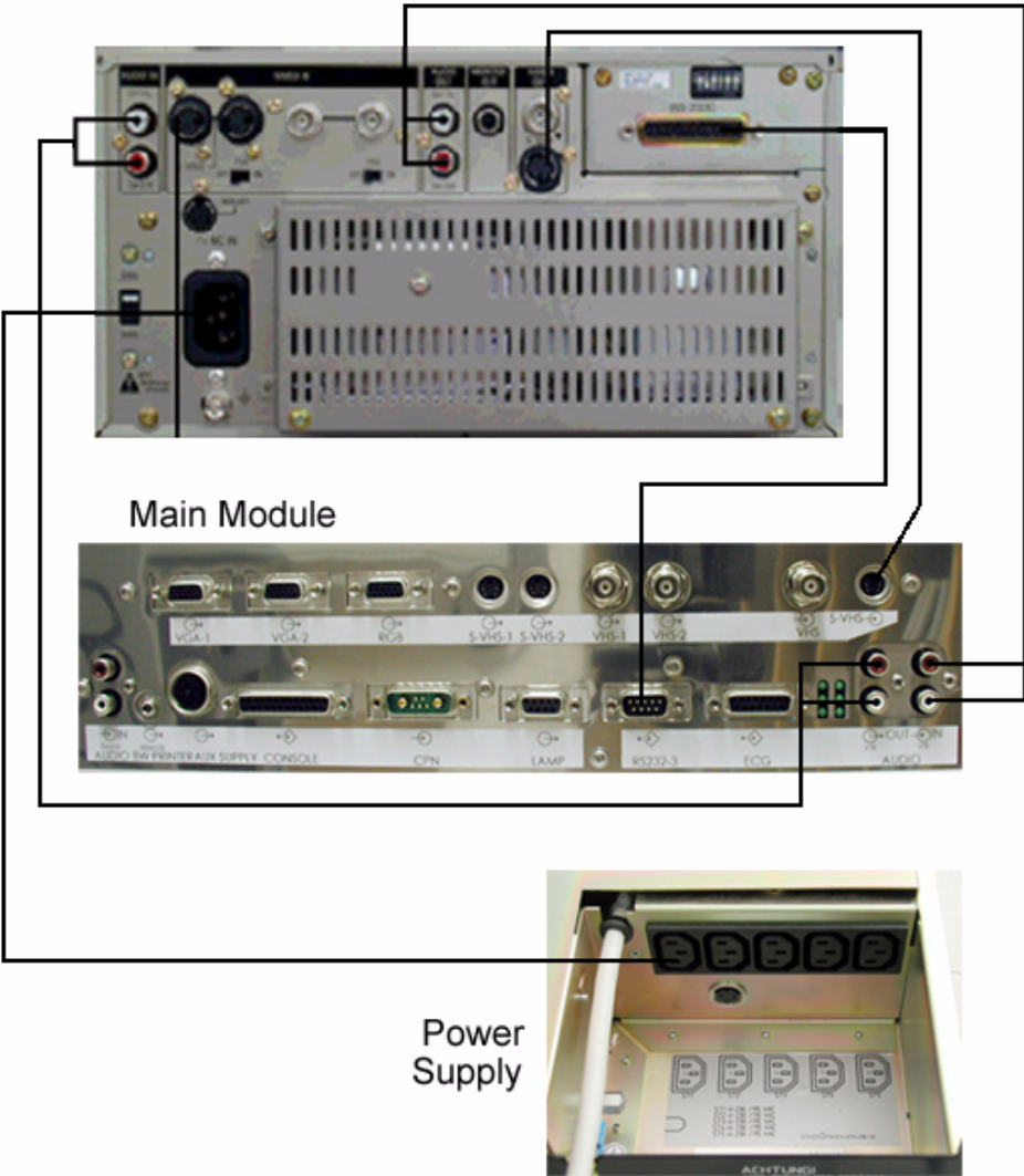
Figure 3-11 Sony - Video Recorder Connection Scheme
