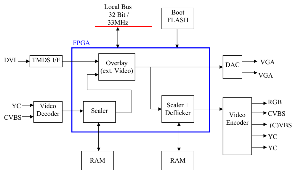
Figure 5-16 Block diagram CKV
