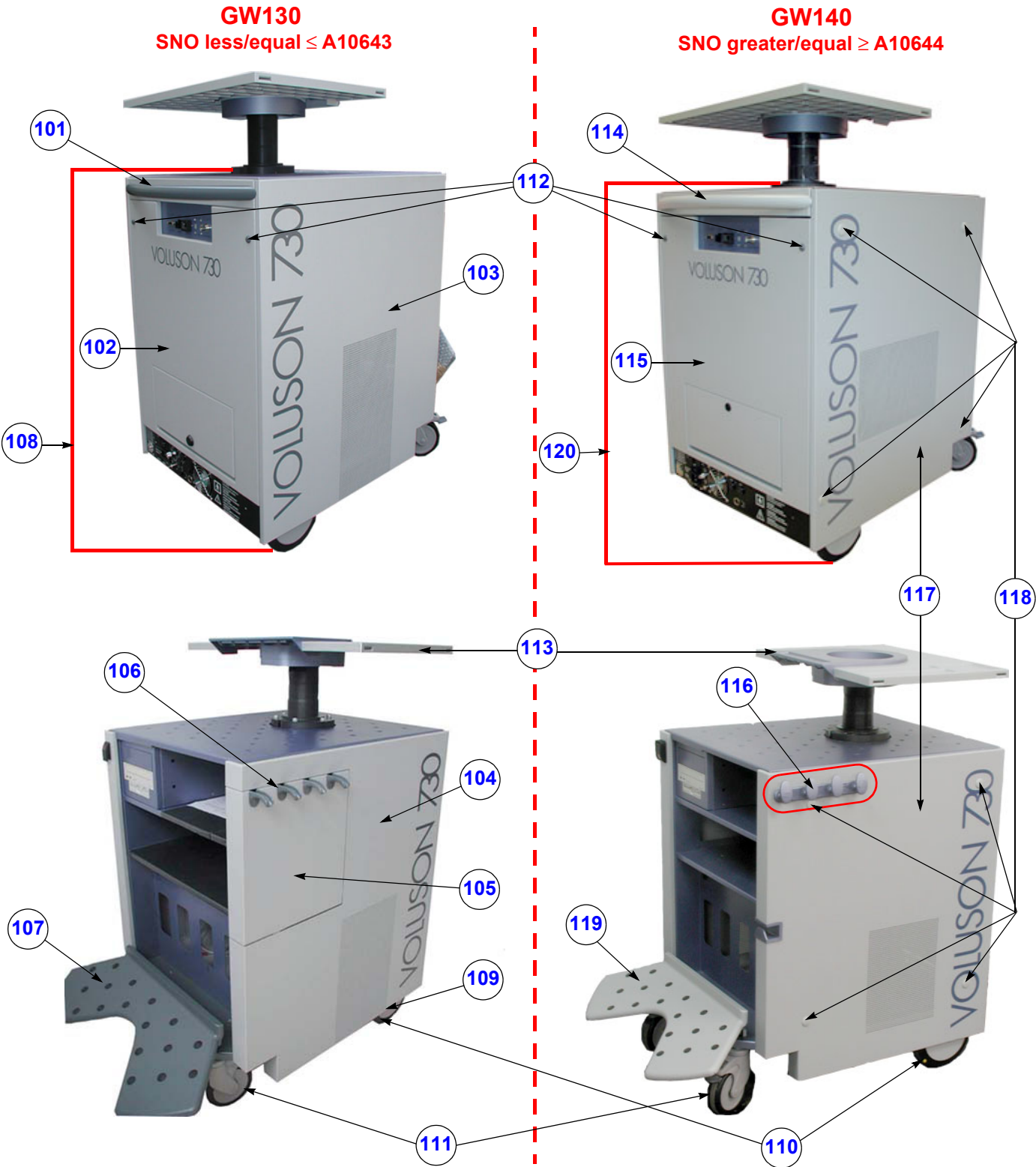
Figure 9-2 Housing (GW)
