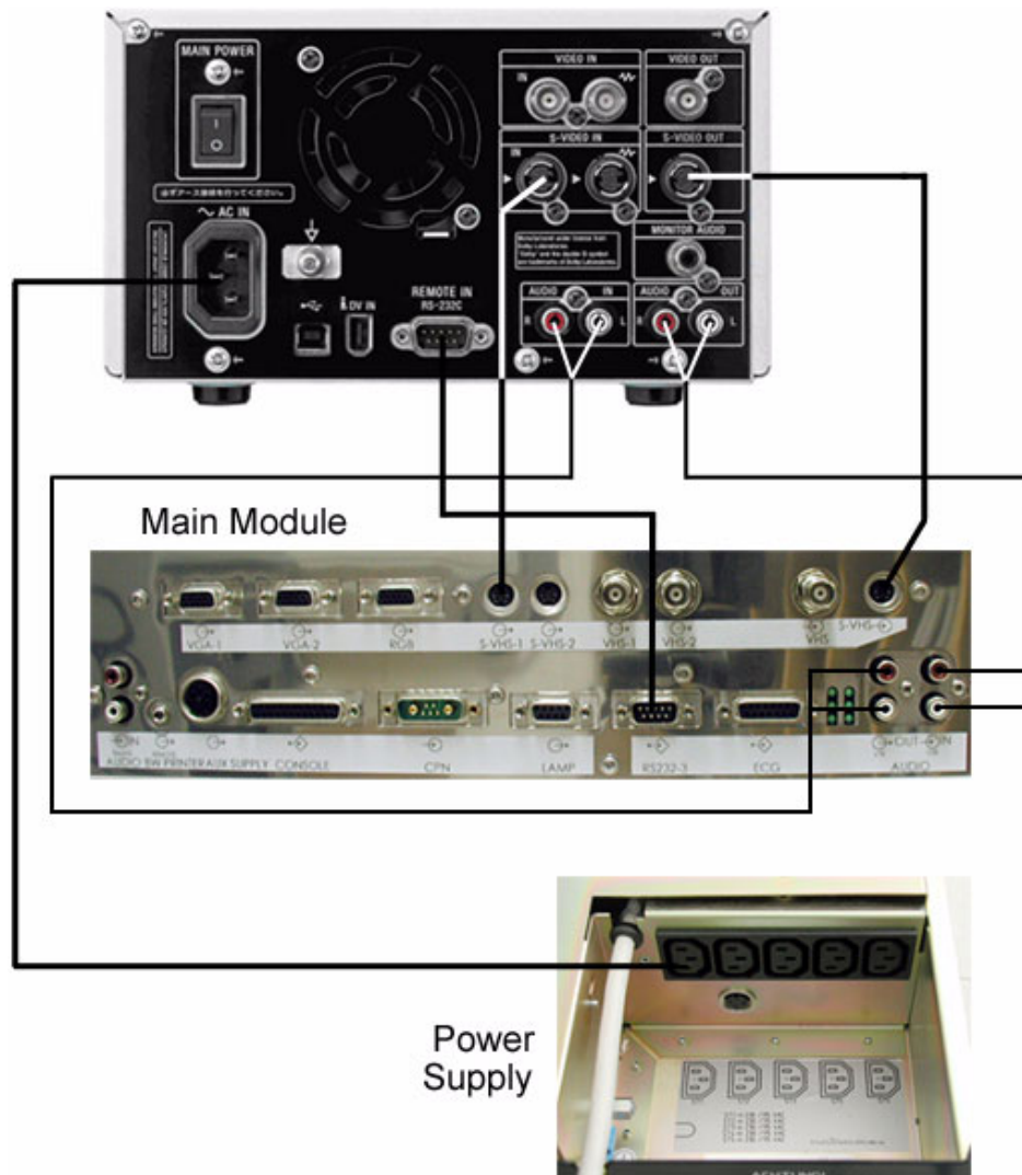
Figure 3-13 DVD Recorder - Connection Scheme
