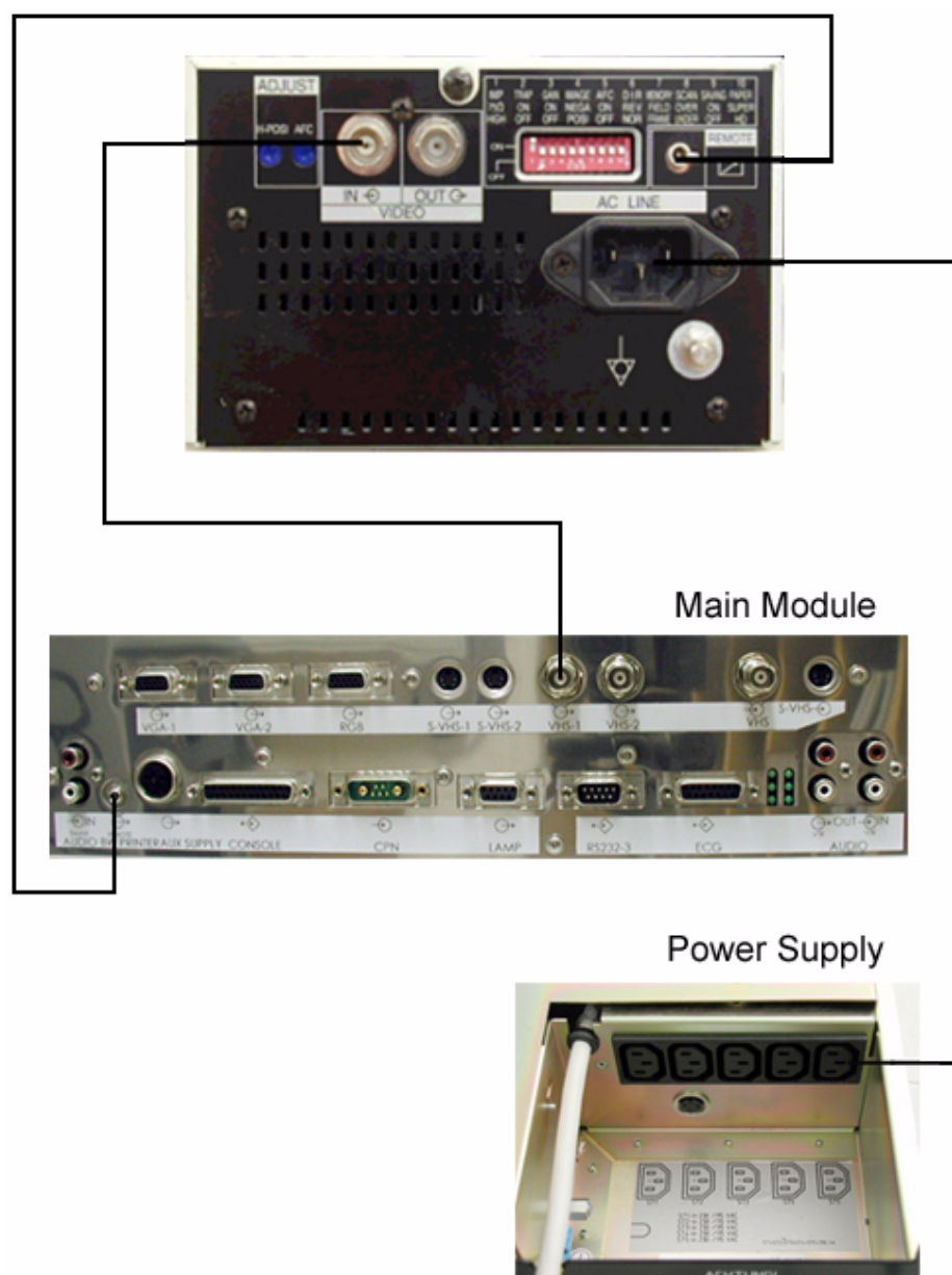
Figure 3-19 B/W Video Printer Connection Scheme
