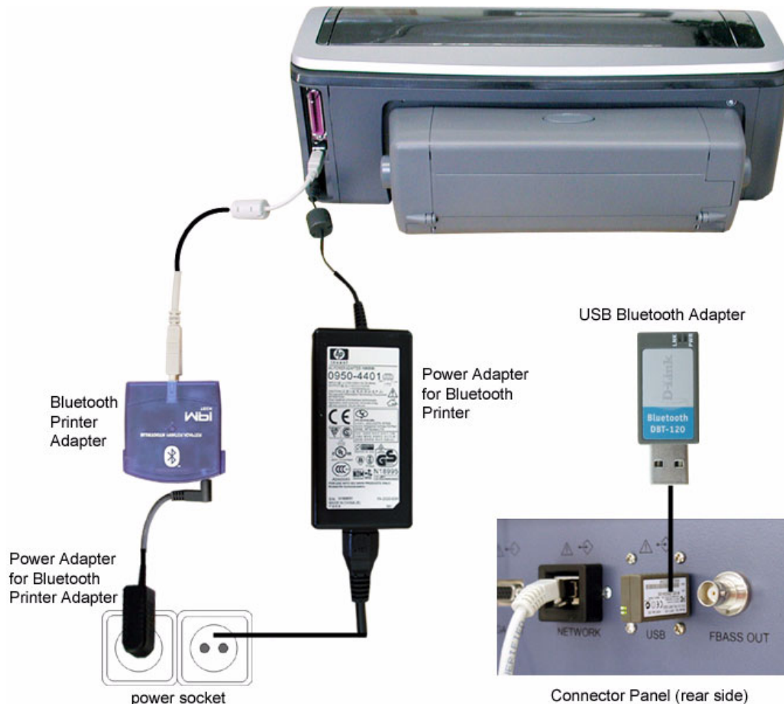
Figure 3-22 HP Bluetooth Printer - Connection Scheme
