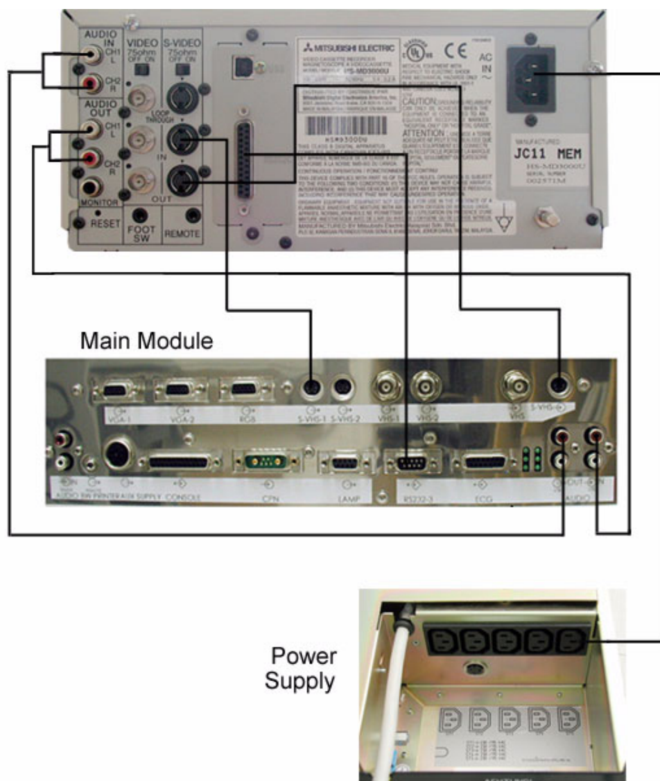
Figure 3-10 Mitsubishi - Video Recorder Connection Scheme
