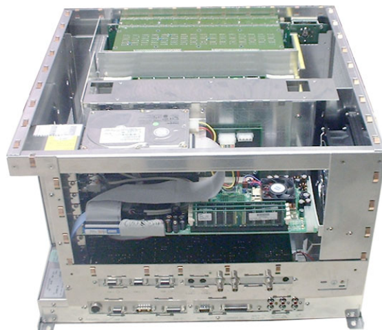
Rear with Internal I/O (Audio Video)
