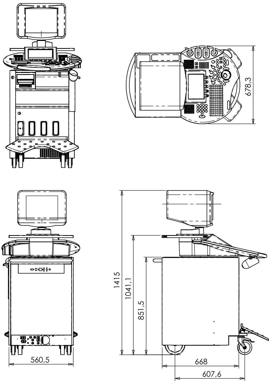
Figure 5-30 Physical Dimensions
