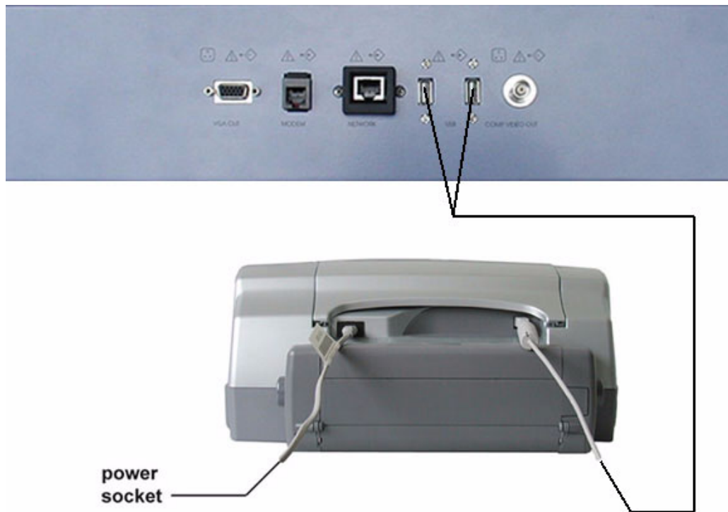
Figure 3-20 Line Printer Connection Scheme
