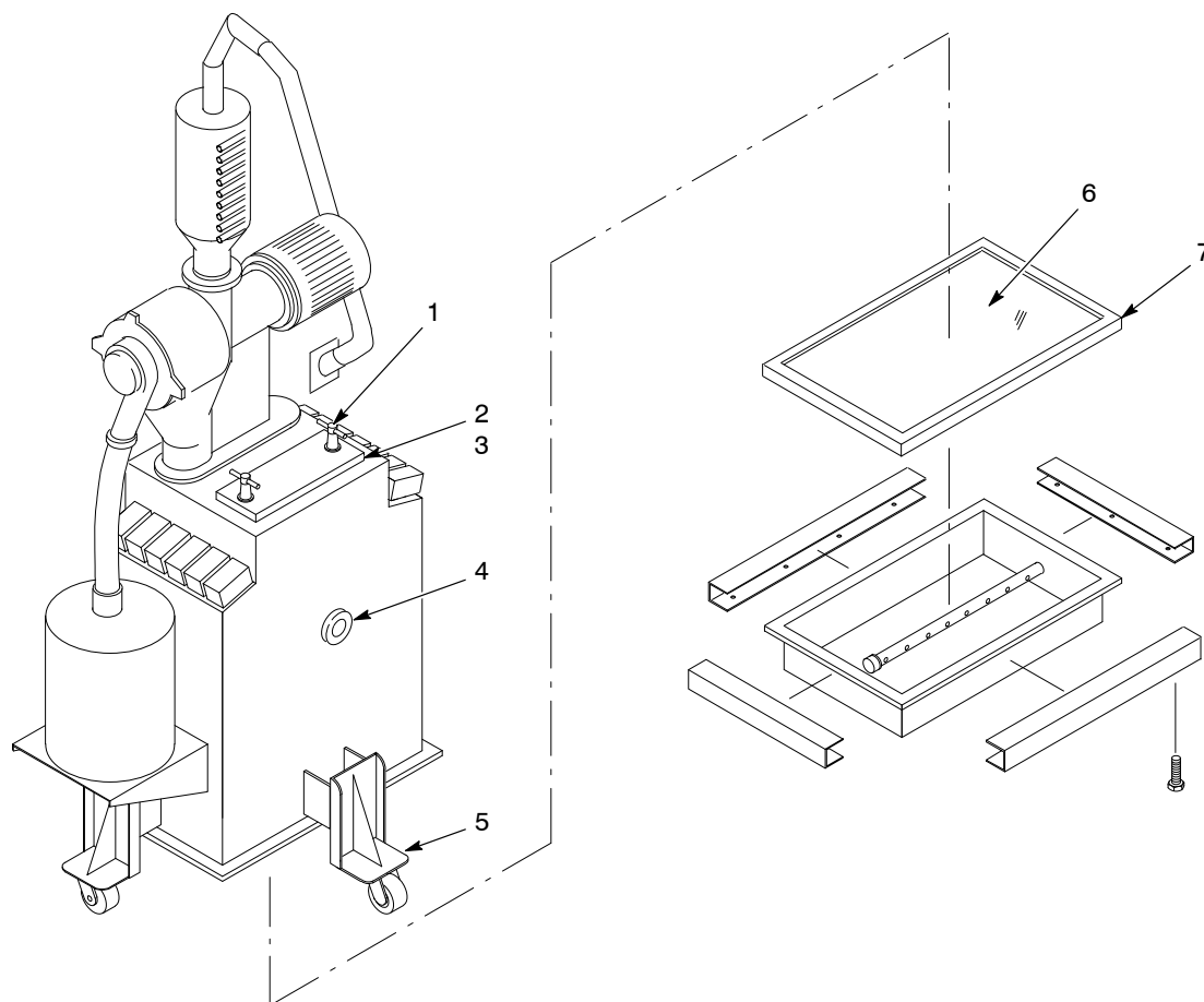
Figure 3 Feed Hopper Parts
