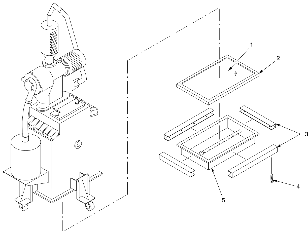
Figure 2 Feed Hopper Fluidizing Plate Replacement
