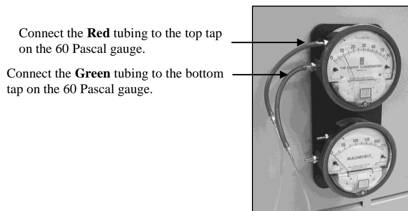
Figure 8: Connecting the Metering Plate to Magnehelic Gauges
