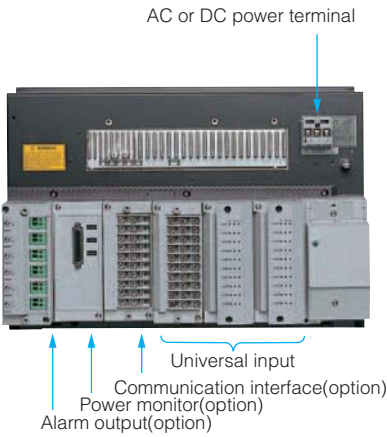
Rear panel of the stand-alone model
