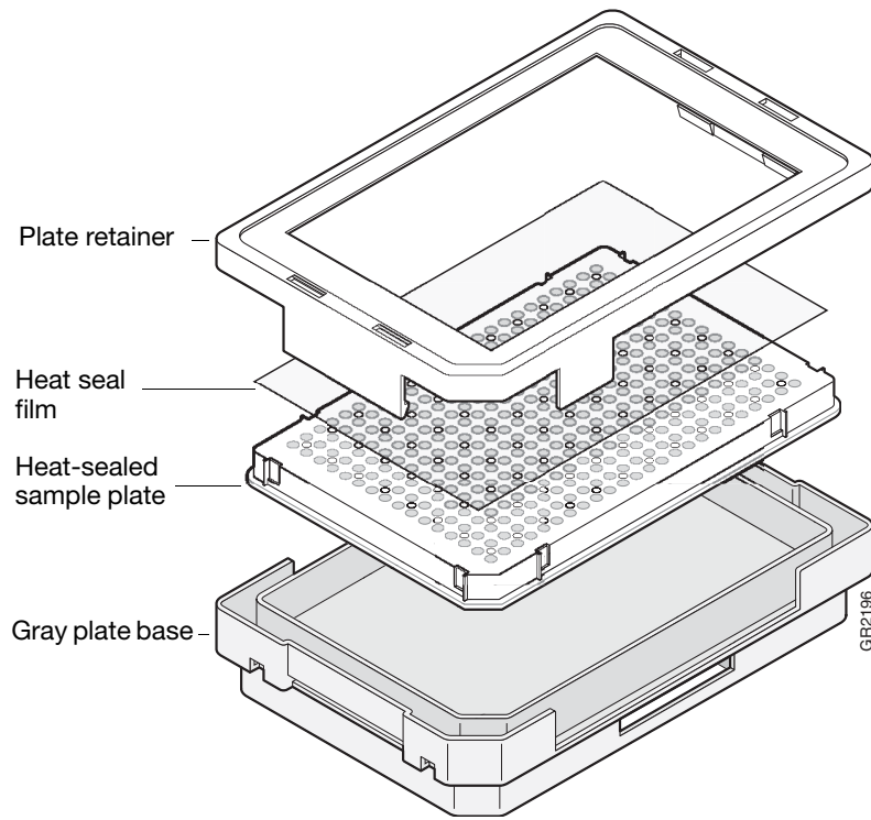
Figure 1-5 Heat Sealed Film Based Plate Assembly
