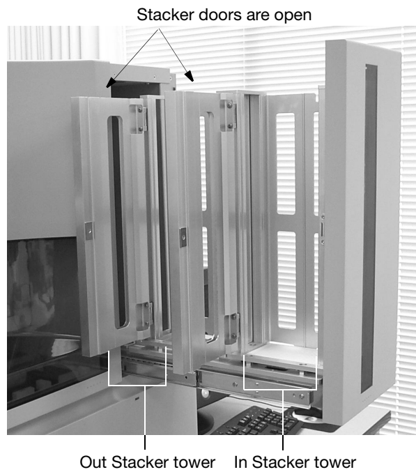
Figure 1-23 Stacker Towers
