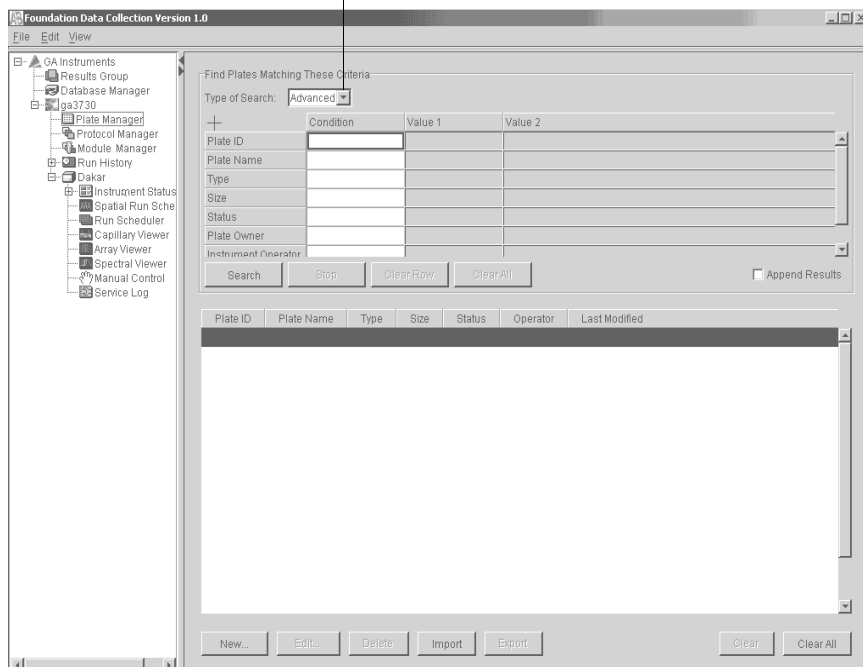
Figure 2-36 Advanced Search Window
