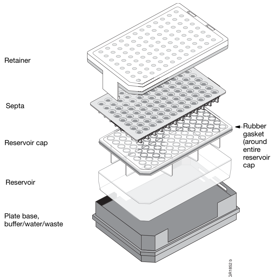
Figure 1-17 Reservoir Assembly
