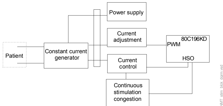
Figure 5 Stimulator block diagram
