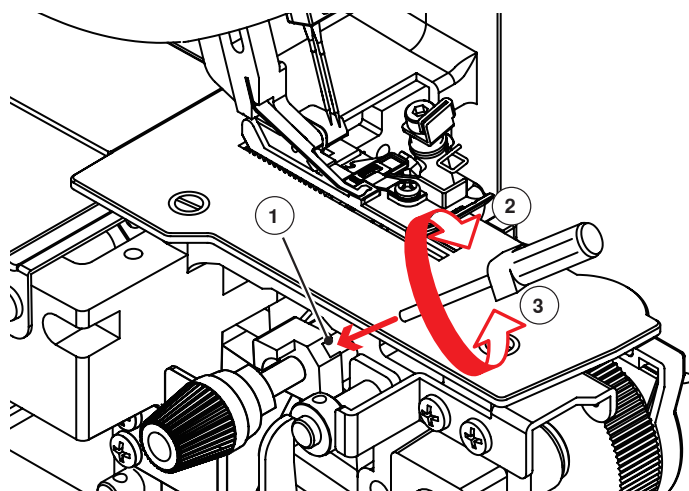
1 Set screw 2 Locking 3 Releasing
