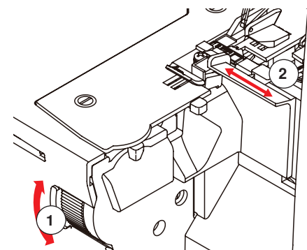
1 Cutting width dial 2 Cutting width indicator
